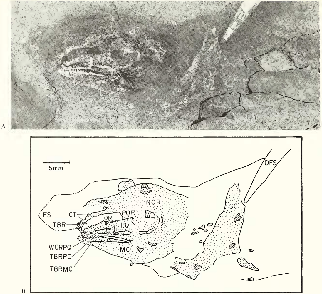
TEXT-FIG. 6. Surcaudalus rostratus n. gen. n. sp. holotype (QMF14470B). A, head and pectoral girdle in lateral view, \times 2.5 . B, drawing of the same specimen.
